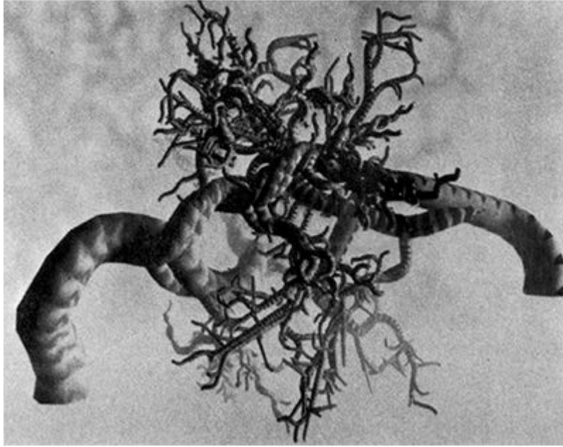
FIGURA 96. The Kiss . (New York Institute of Technology [Peter Oppenheimer].)
